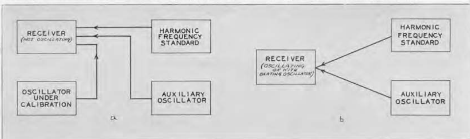
FIGURE 2. (a) Block diagram showing the process of calibrating an oscillator by means of an auxiliary oscillator set to the desired frequency span. (b) A similar system for calibrating a receiver.
