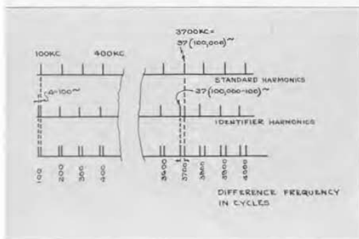
FIGURE 4. Showing operation of identifier.
