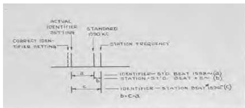
FIGURE 5. Showing use of identifier in avoiding very low beat frequencies in measuring a radio frequency very near a standard harmonic.
