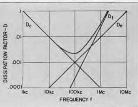
FIGURE 8. Component dissipation factors of an air-cored coil; D_c from ohmic resistance, D_e from eddy currents, and D_f from distributed capacitance.
