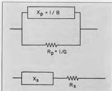
FIGURE 3 (above). Parallel components of a reactor.
