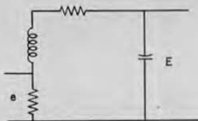
FIGURE 6. Circuit for measuring step-up voltage ratio.
