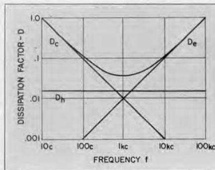
FIGURE 7. Component dissipation factors of an iron-cored coil; D_c from ohmic resistance, D_h from hysteresis, and D_e from eddy currents.
