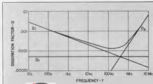
FIGURE 5. Component dissipation factors of a mica capacitor; D_i from interfacial polarization, D_r from residual polarization, and D_s from series resistance.
